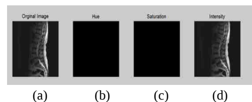
Fig. 8: HSI Components
