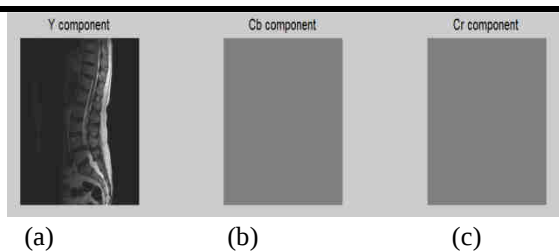
Fig. 5: YCBCR Components
